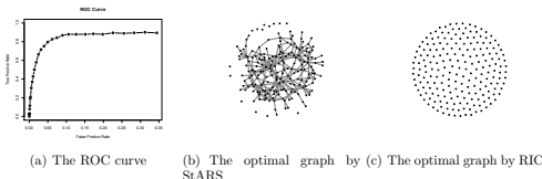
Figure 2: Simulated results w/o nonparanormal
