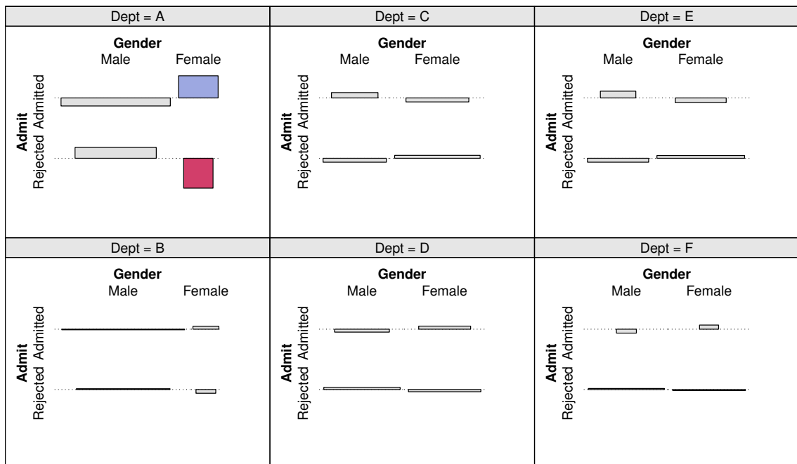
Figure 2: Conditional association plot for the UCBAmissions data.
